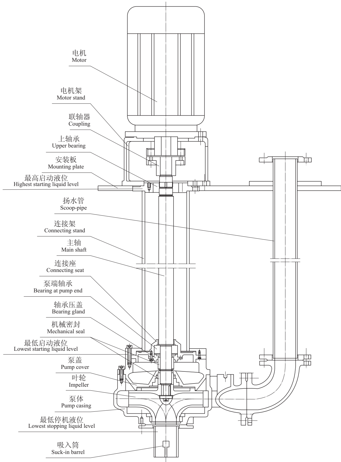
YW(P)液下排污泵结构示意图 Table of YW(P) series under-liquid sewage pump's structure drawing
